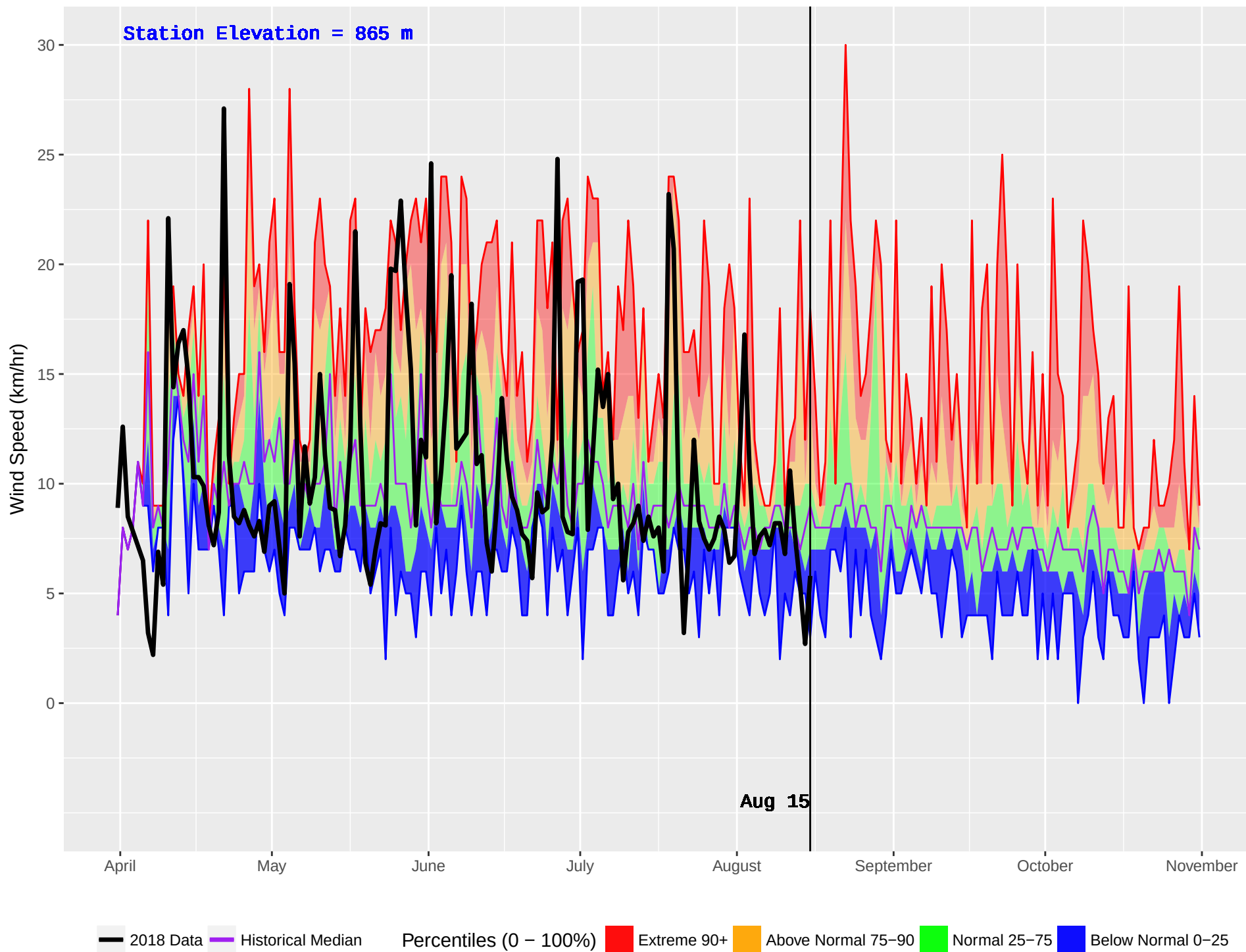
FIVE MILE (1029) : Historical (2008–2016) and Current (2018) Daily Wind Speed
