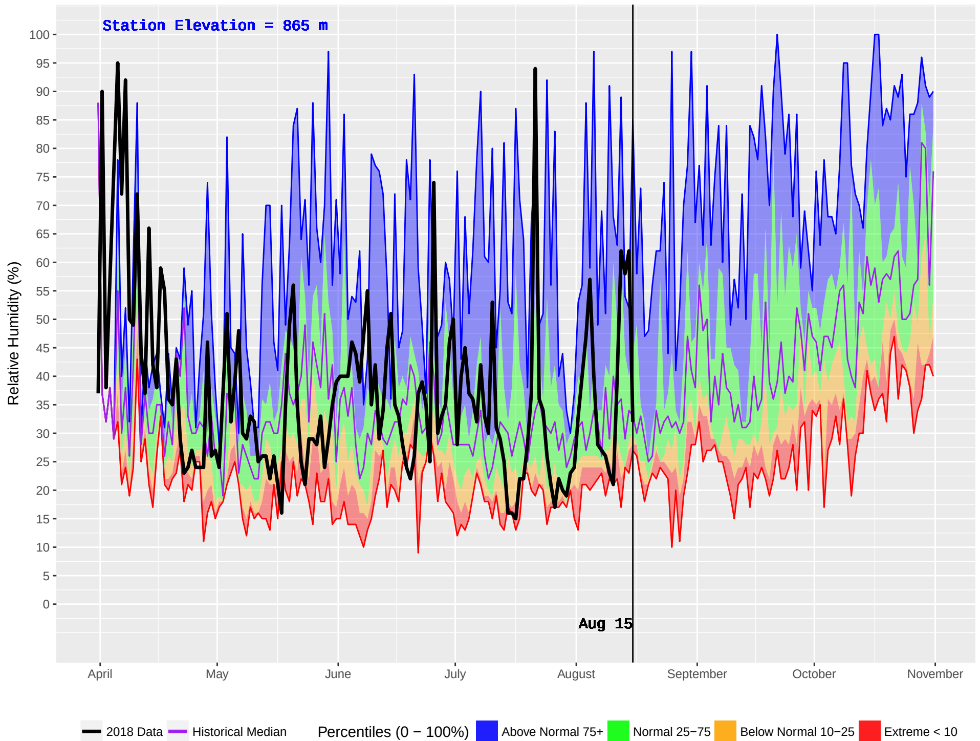
FIVE MILE (1029) : Historical (2008–2016) and Current (2018) Daily Relative Humidity
