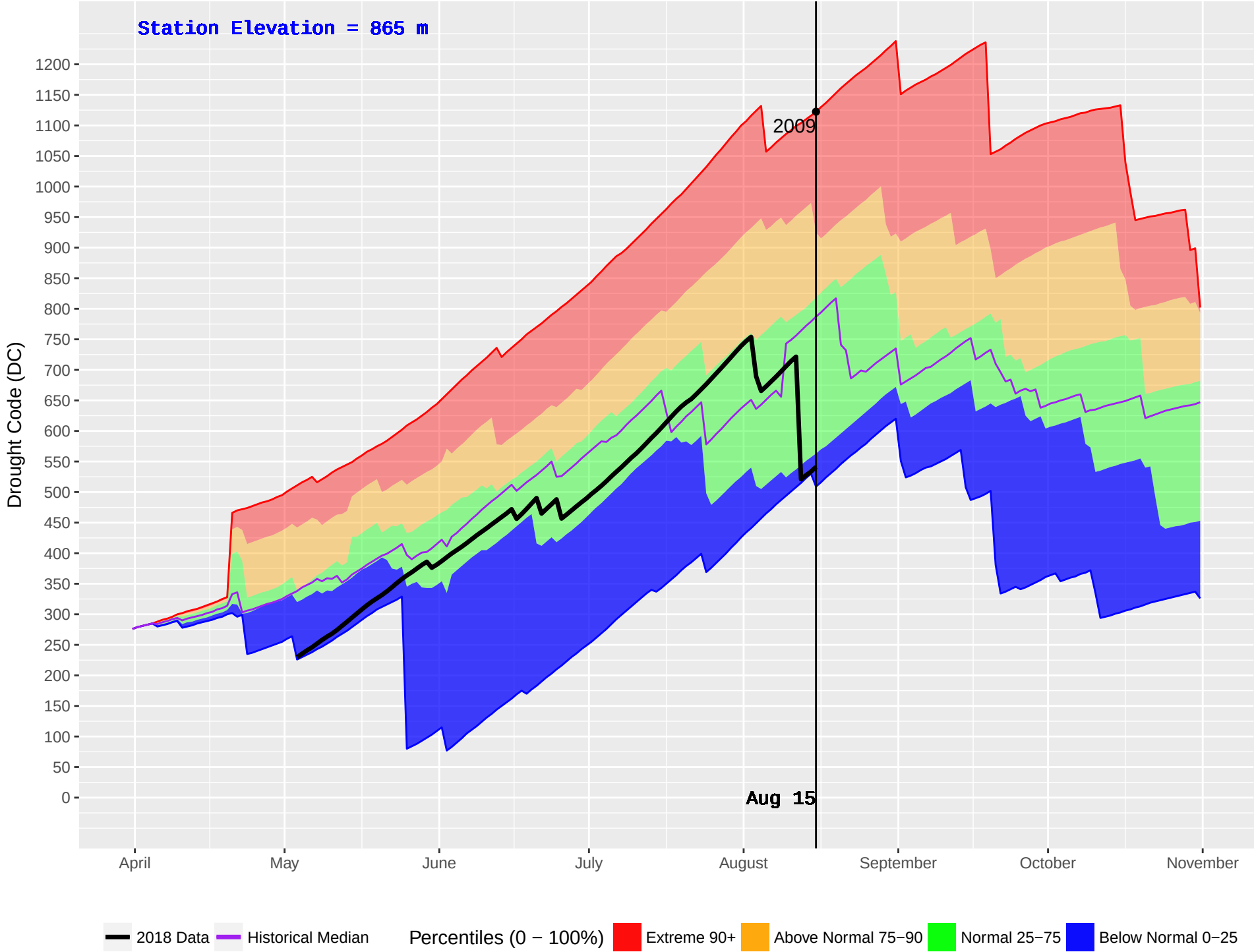
FIVE MILE (1029) : Historical (2008–2016) and Current (2018) Daily Drought Code (DC)
