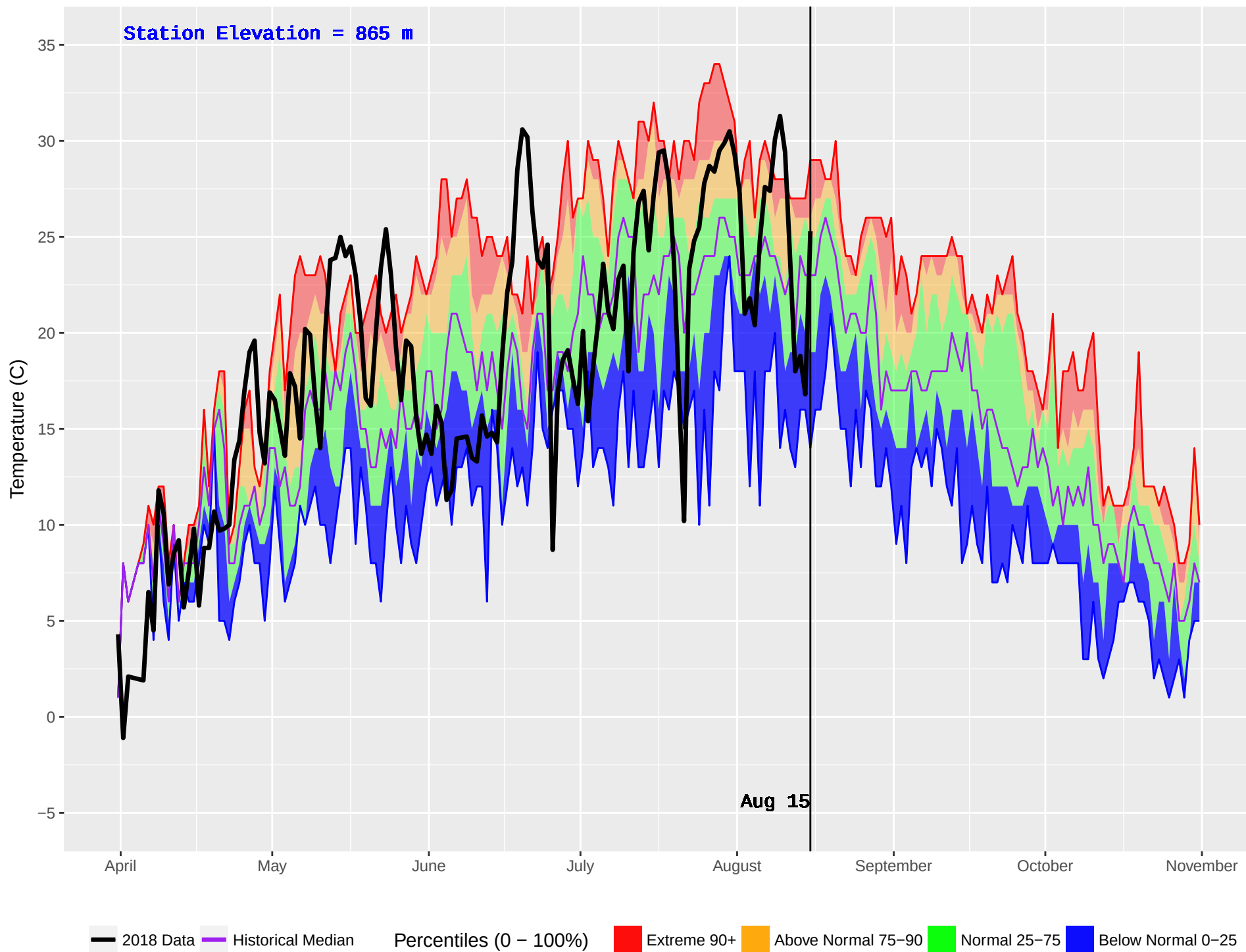
FIVE MILE (1029) : Historical (2008–2016) and Current (2018) Daily Temperature
