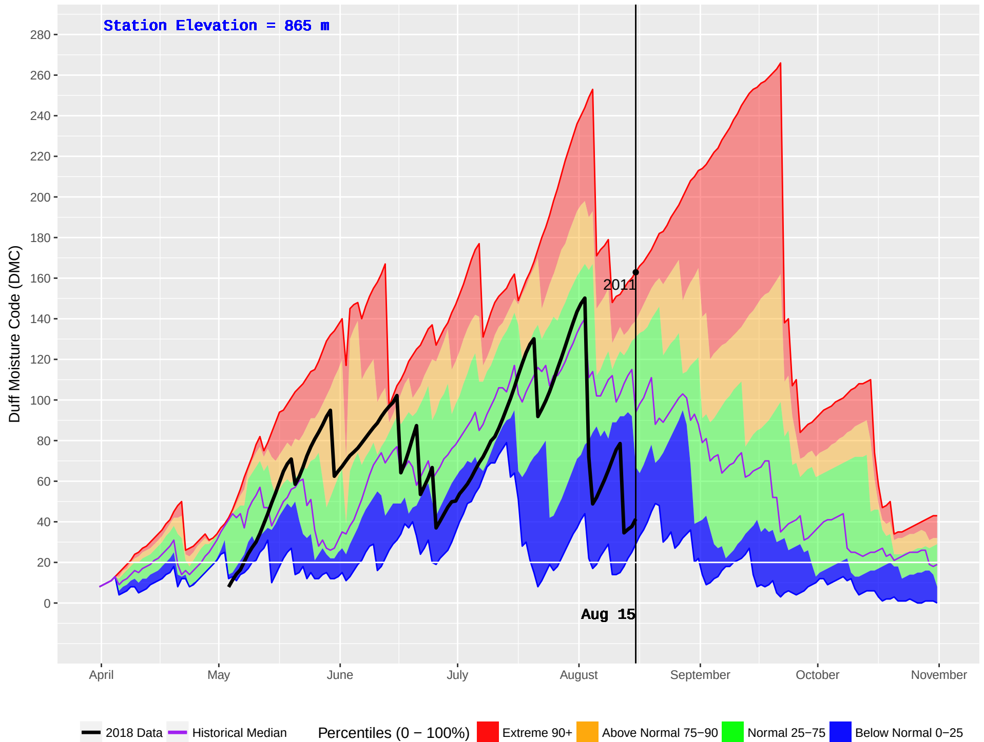
FIVE MILE (1029) : Historical (2008–2016) and Current (2018) Daily Duff Moisture Code (DMC)
