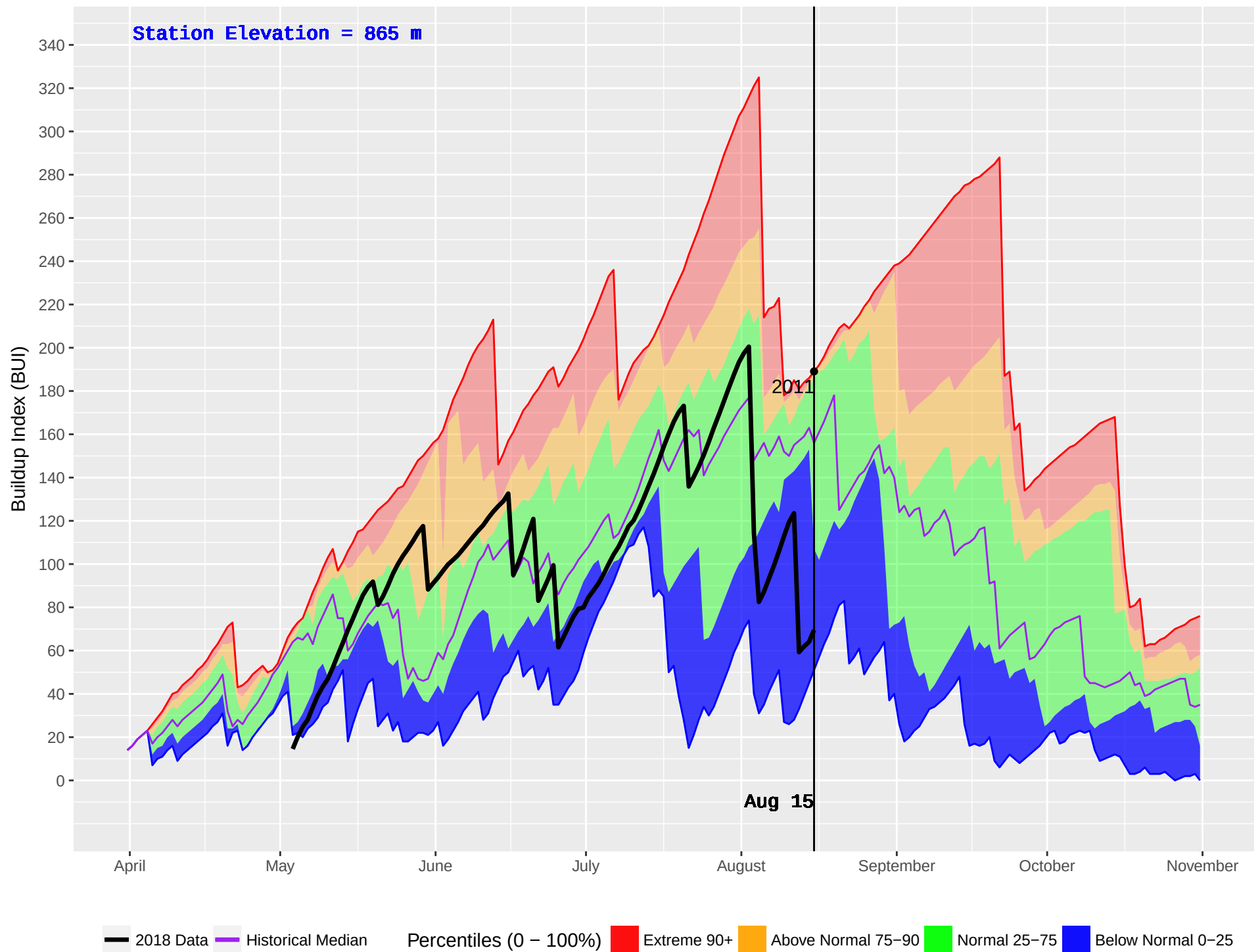
FIVE MILE (1029) : Historical (2008–2016) and Current (2018) Daily Buildup Index (BUI)
