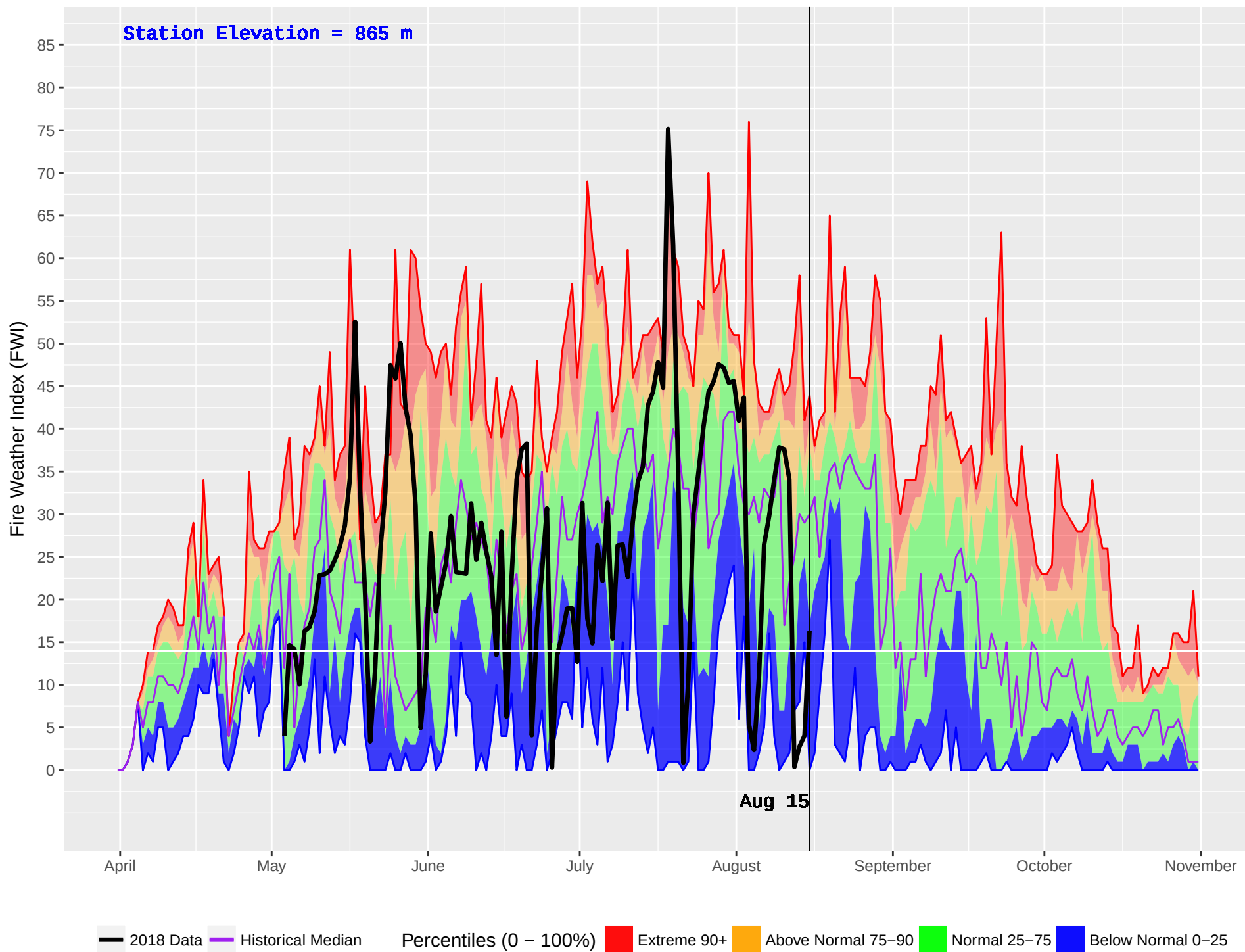
FIVE MILE (1029) : Historical (2008–2016) and Current (2018) Daily Fire Weather Index (FWI)
