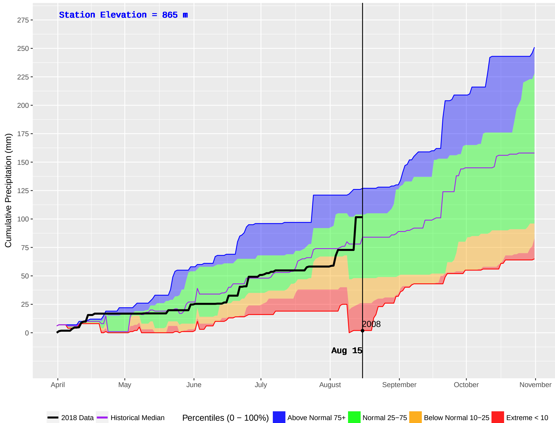
FIVE MILE (1029) : Historical (2008–2016) and Current (2018) Daily Cumulative Precipitation
