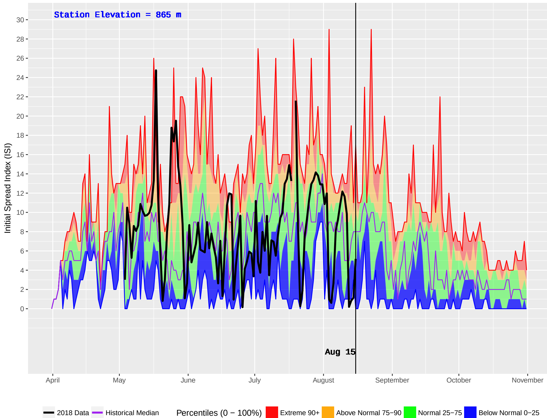
FIVE MILE (1029) : Historical (2008–2016) and Current (2018) Daily Initial Spread Index (ISI)
